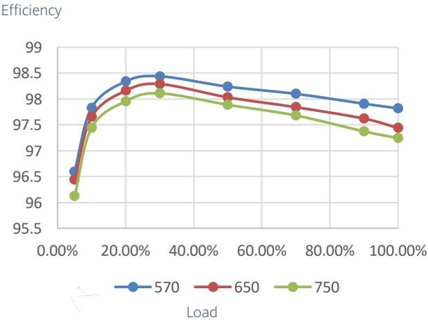
Efficiency Curve
